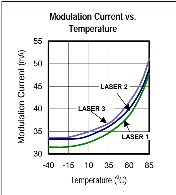
Figure 11. Modulation Current vs. Temperature
