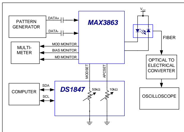
Figure 6. Setup Diagram
